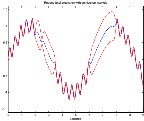
Fig. 3. Prediction and confidence interval with long and short length scale components.
