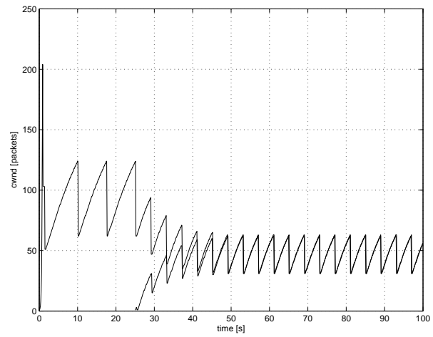
Figure 9. Two sources competing for bandwidth with \alpha_i = 1 , \beta_i = 0.5 . 95% convergence is achieved in 4 congestion epochs. (NS simulation results, network parameters: 10Mb bottleneck link, 100ms delay, queue 40 packets)
