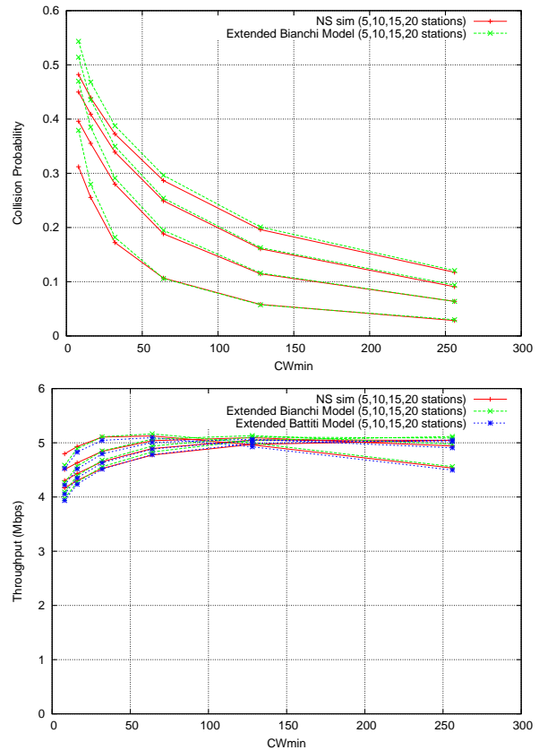
Figure 5. 802.11e theory versus simulation, varying numbers of upload flows, topology as in Figure 2, delayed acking used in TCP sink (which is in the access point).
