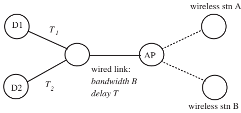
Figure 6. Network topology used to compare characteristics of TCP uploads with wired/wireless bottleneck link. (Network parameters: T = 10ms , T_1 = 0ms , T_2 = 40ms , wired link queue 0.0001B , 802.11b PHY, TCP uploads from stn A to D1 and from stn B to D2.)
