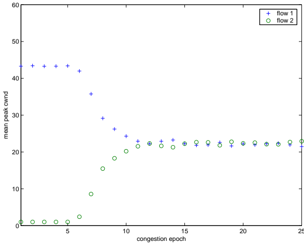
(a) \beta_2=0.5
