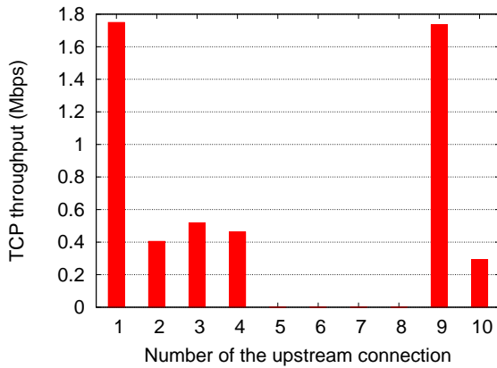
Figure 1. Throughput of competing TCP uploads (NS simulation, 10 upload TCP flows, single cell infrastructure mode 802.11b WLAN, TCP SACK).
