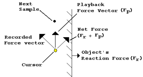
Figure 2: Demonstration of the problems of playback when the cursor and next sample point lie inside an object. The direction of the playback force will be affected by the object's reaction force and resultant force will push the cursor away from the sample point.
