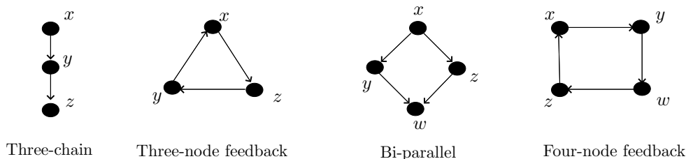
Figure 5: Common motifs in real networks
