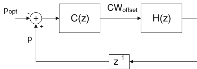
Figure 1 Control system
