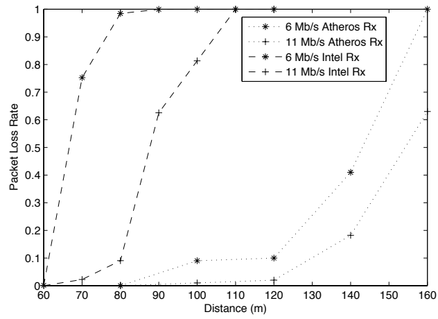
Fig. 3. Measured PLR vs. distance in day-time outdoor environment. Experiment
