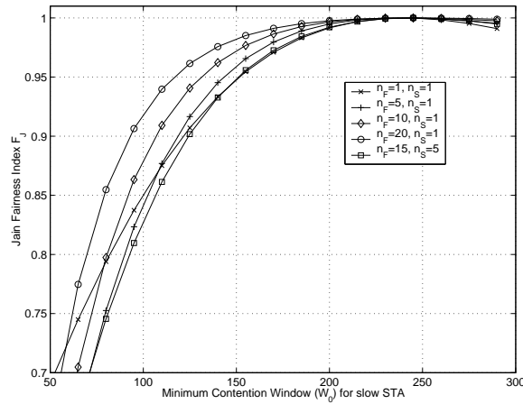
Figure 8: Fairness of time allocation for different W_0 of the slow STA. W_{max} of the slow STA is dynamic. W_0 of the fast STAs is fixed to 32. All STAs have a payload size of 1470 bytes and are saturated.
