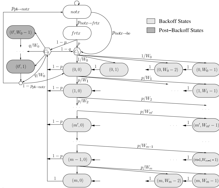
Figure 2: Finite load source model for DCF
