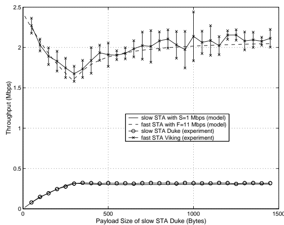
Figure 5: Throughput for a fast and a slow STA. The fast STAs are saturated with a fixed payload size of 1470 bytes. The data rate for the slow STA Duke is limited to 320Kb/s.
