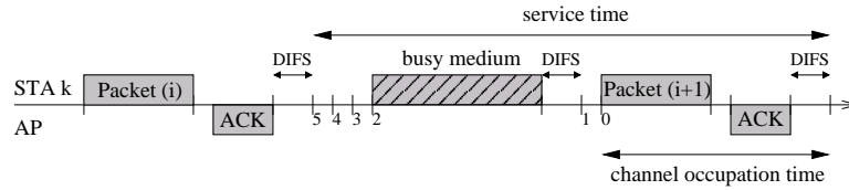
Figure 6: Service time and channel occupation time.
