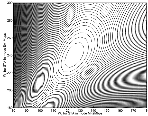
Figure 13: Contour plot for the fairness of time allocation for different W_0 of STAs in modes S and M . W_0 of the fast STA is fixed to 32. All STAs have a payload size of 1470 bytes and are saturated ( n_S = n_M = n_F = 1 ).
