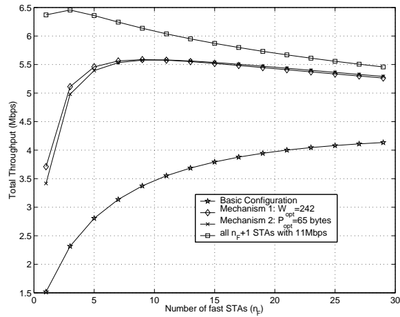
Figure 10: Total throughput versus number of fast STAs. All STAs are saturated.
