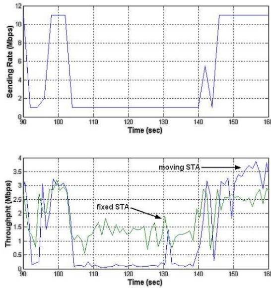
Figure 1: The throughput of one fixed STA and one moving STA.
