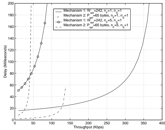
Figure 11: MAC layer delay for the slow STA using either Mechanisms 1 or 2. The fast STAs are saturated and use a payload size of 1470 bytes.
