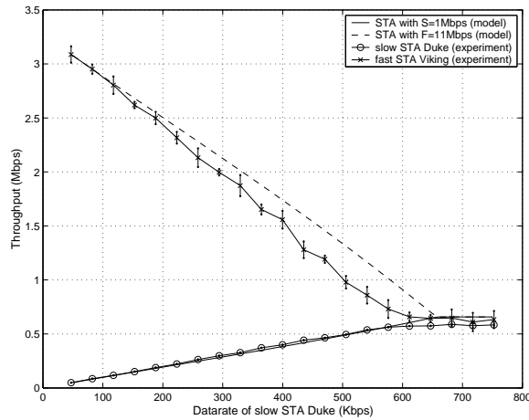
Figure 4: Throughput comparison between model and experiment when we vary the data rates. The saturation throughput of Viking is slightly overestimated in our model, which is mainly caused by the perfect medium assumption.
