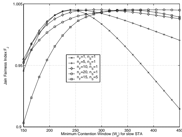
Figure 9: Fairness of time allocation for different W_0 of the slow STA. W_{max} is static fixed to 1024 for all STAs.
