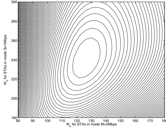
Figure 14: Contour plot for the fairness of time allocation for different W_0 of STAs in modes S and M . W_0 of the fast STAs (mode F ) is fixed to 32 ( n_S = 4 , n_M = 6 and n_F = 8 ).
