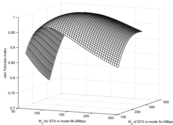
Figure 12: Fairness of time allocation for different W_0 of STAs in modes S and M . W_0 of the fast STAs is fixed to 32. All STAs have a payload size of 1470 bytes and are saturated.
