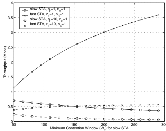
Figure 7: Saturation throughput for the fast and slow STAs with different W_0 of the slow STA. All STAs have a packet size of 1470 bytes. W_0 of the fast STA is fixed to 32.
